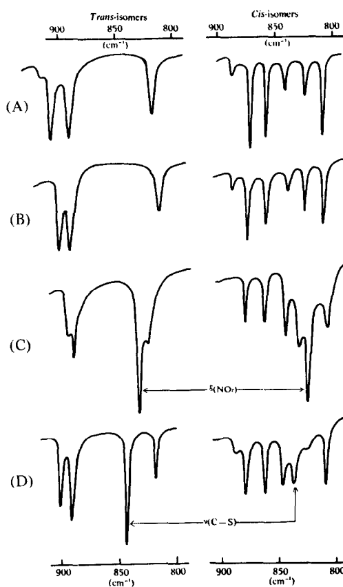
Figure 1. Infrared Spectra in the 800-910 cm -1 region of some cis - and trans - cobalt(III) cyclam complexes.
